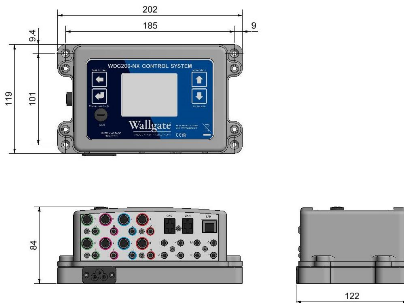
Figure 7. WDC200-NX Dimensions
